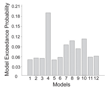
Figure 5. a, b , The optimal model selected by the FFX analysis ( a ) and RFX analysis ( b ). The left graph in each analysis showed the parameters for the optimal model, model 4. Values are the across-subjects mean (SD) of rate constants for intrinsic connections, direct effects of extrinsic inputs, and modulatory effects on a certain connection, estimated by DCM10 ( p < 0.05 in t test indicated by solid lines). The right graph in each analysis showed the results of Bayesian model selection. The relative group model evidence ( a ) and model exceedance probability ( b ) is the highest for model 4.
