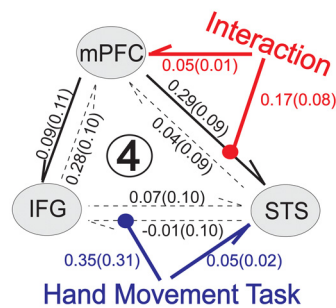
Figure 5. a, b , The optimal model selected by the FFX analysis ( a ) and RFX analysis ( b ). The left graph in each analysis showed the parameters for the optimal model, model 4. Values are the across-subjects mean (SD) of rate constants for intrinsic connections, direct effects of extrinsic inputs, and modulatory effects on a certain connection, estimated by DCM10 ( p < 0.05 in t test indicated by solid lines). The right graph in each analysis showed the results of Bayesian model selection. The relative group model evidence ( a ) and model exceedance probability ( b ) is the highest for model 4.
