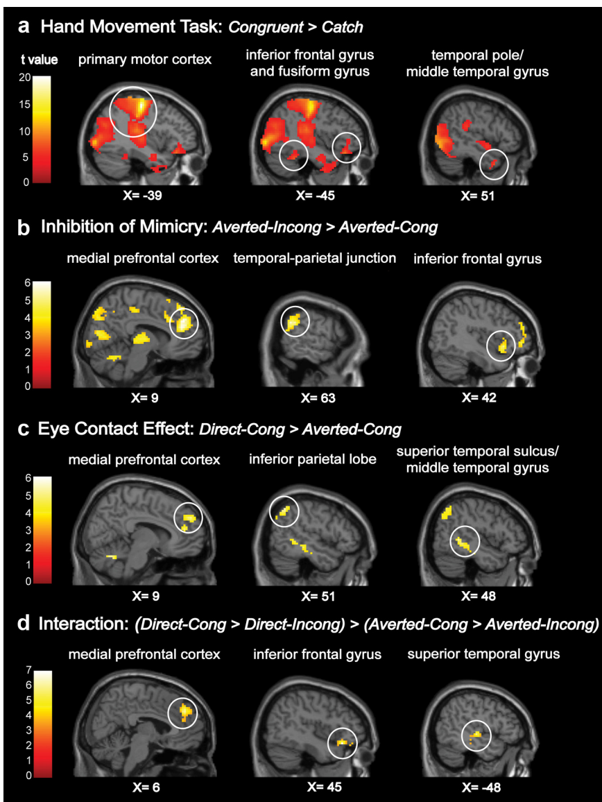
Figure 2. a–d , Brain regions showing increased activations for the hand movement task ( a ), the simple effect of inhibition of mimicry ( b ), the simple effect of eye contact ( c ), and the interaction of gaze and mimicry ( d ). Coordinates are listed in Table 1.
